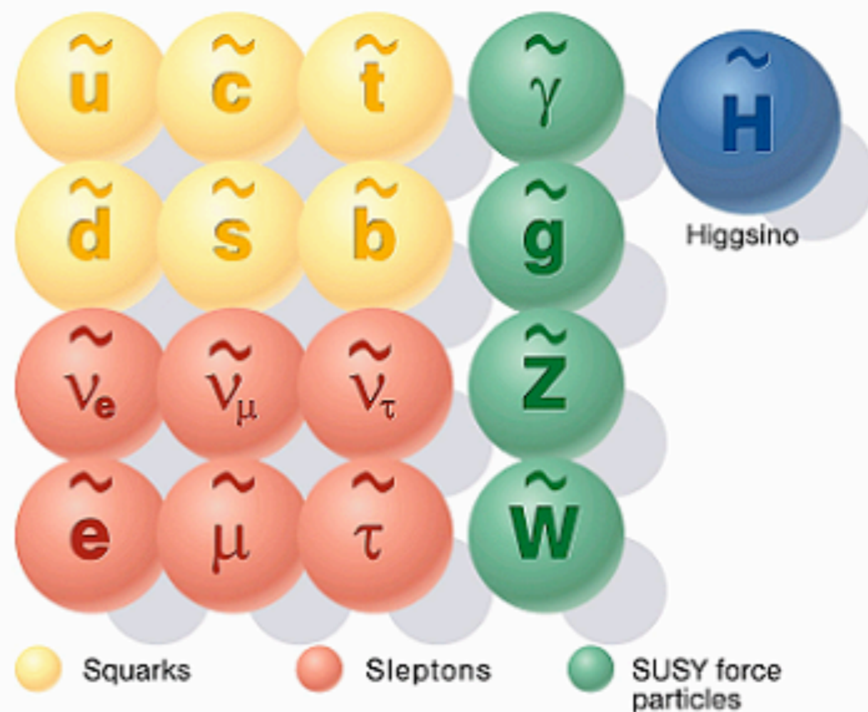
SUSY particles
